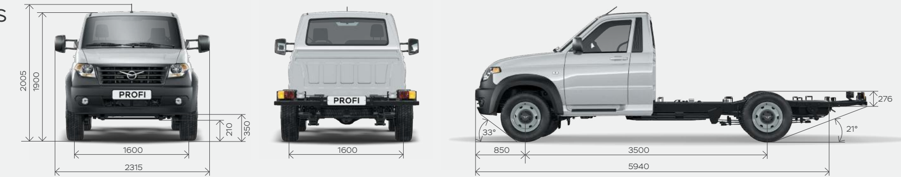
Chassis cab
